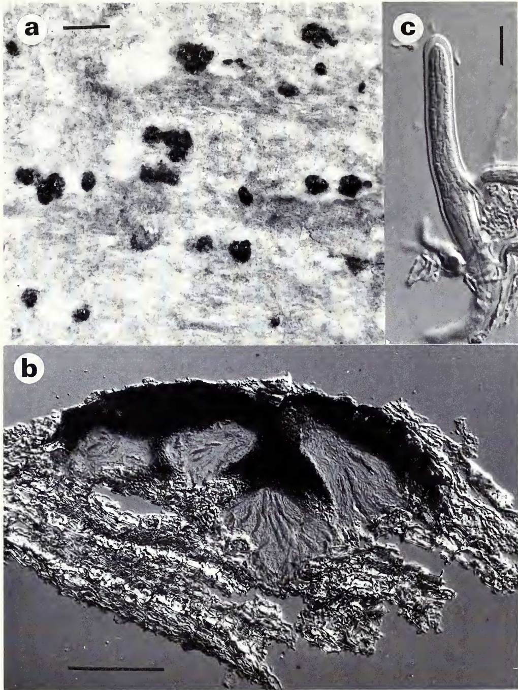
Fig. 35 Celothelium dominicanum (Vainio) Aguirre (TUR 32697–holotype) (a) Surface view of ascomata; scale = 500 \mu\text{m} ; (b) Vertical section of ascomata; scale = 100 \mu\text{m} ; (c) Ascus and ascospores; scale = 10 \mu\text{m} .
